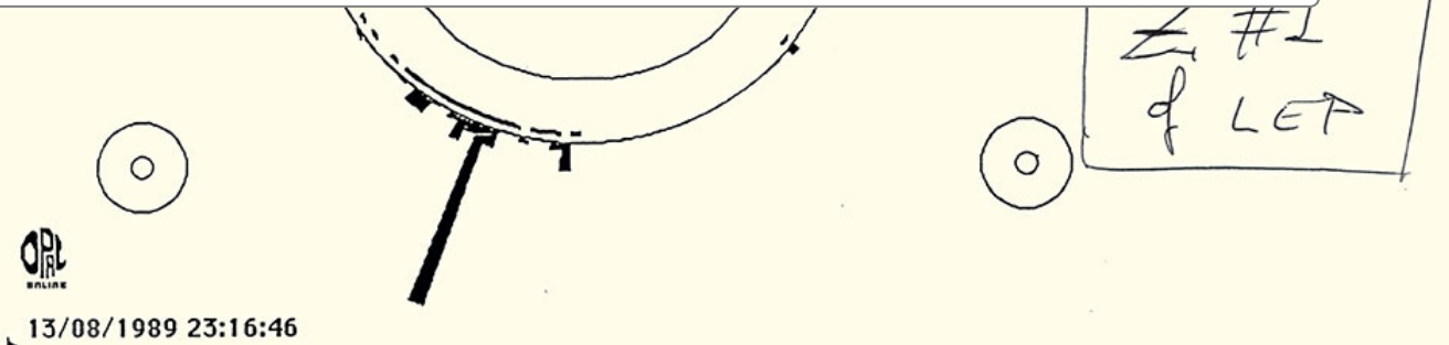
OPAL logbook entry on 13 Aug 1989 with the first Z-boson candidate
