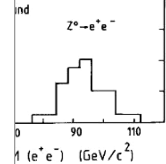
Mass spectrum of all e^+e^- pairs measured by UA1 in 1982-1985
