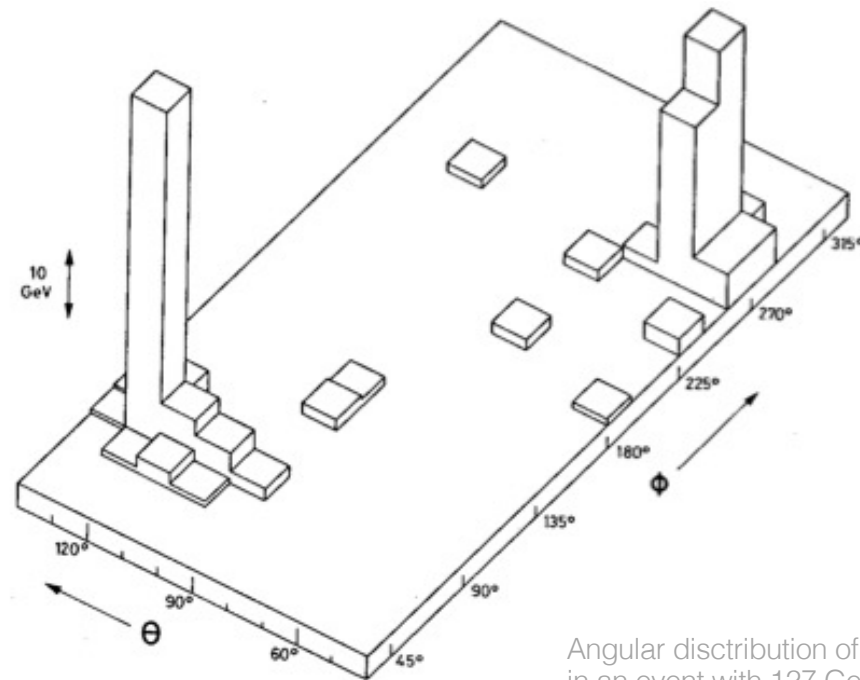
First observation of high- p_T jets at hadron collider (UA2, ICHEP 1982)
