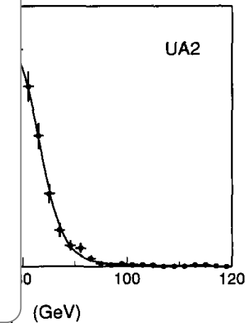
Jacobian peak with full UA2 dataset (1992): m_W = 80.84 \pm 0.22 GeV
