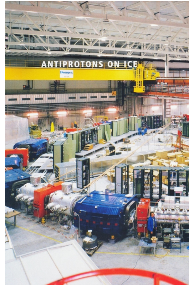
Antiproton Accumulator (antiprotons produced in PS at \sim 3.5 \text{ GeV} ; it took about 20 hours of stacking and cooling to produce a sufficiently dense antiproton stack for transfer to SPS)
